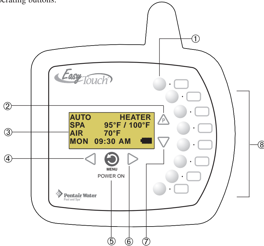
EasyTouch Wireless Control Panel (eight circuit)
